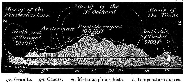
FIG. 5.—Section across St. Gothard (reduced from the large section of Dr. Stapff).
