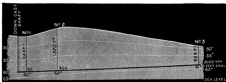
FIG. 4.—Section at Vochriw Dowlais, Aberdare District.
