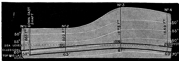
FIG. 3.—Section at New Tredegar, Aberdare District.
