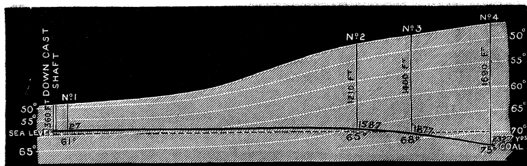
FIG. 1.—Section at Upper Duffryn, Aberdare District.
